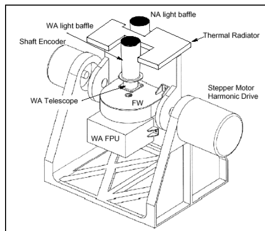
Figure 5. MDIS design.
