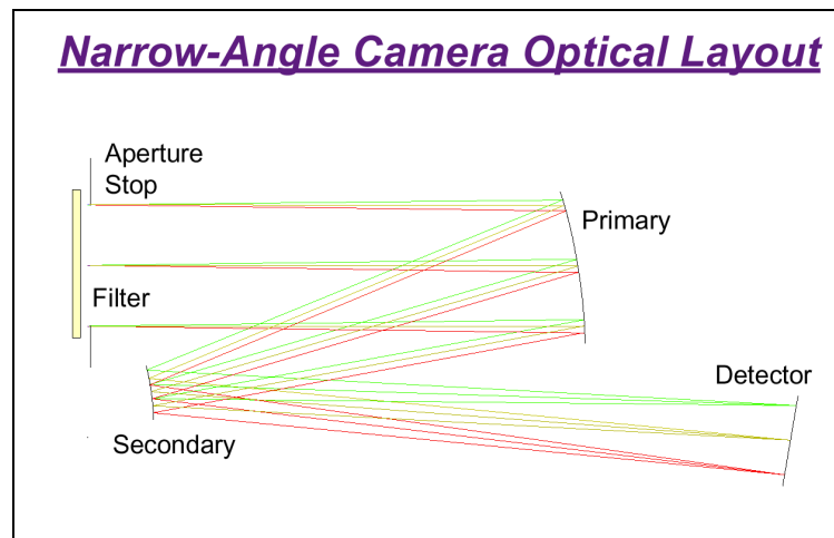
Figure 10. NAC optical layout.
