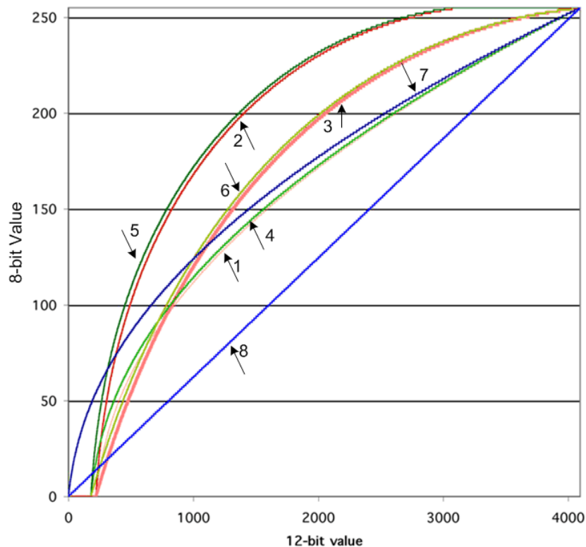
Figure 8. Mapping of 12 bits to 8 bits will be accomplished using onboard look-up tables. The tables are designed to preferentially preserve information at different DN ranges, and they can accommodate a nominal detector dark level as well as one that has changed with time. (1) Low noise, high bias SNR proportional. Usage: Typical imaging with varied brightness. (2) Low noise, high bias DN-weighted SNR proportional. Usage: Faint object imaging. (3) High noise, high bias DN-weighted SNR proportional. Usage: B/W, low brightnesses. (4) Low noise, medium bias SNR proportional. (5) Low noise, medium bias DN-weighted SNR proportional. Usage: Faint objects. (6) High noise, medium bias DN-weighted SNR proportional. Usage: B/W mostly low brightness. (7) Zero-bias SNR proportional. Usage: Typical imaging, varied brightness. (8) Linear. Usage: High brightness mapping, preserves high DN information.
