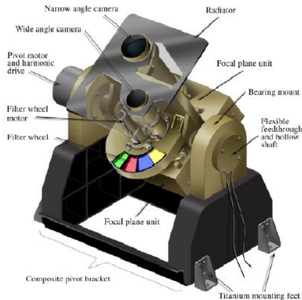
Figure 1: CAD rendering of MDIS instrument.
