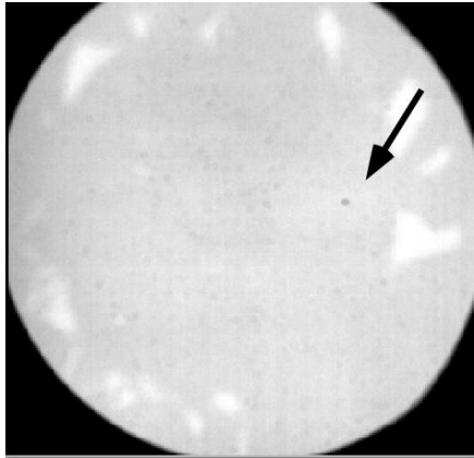
Figure 12: Non-uniformity due to dust particles is visible in integrating sphere images acquired through the quartz window in the OCF chamber door of the calibration facility.
