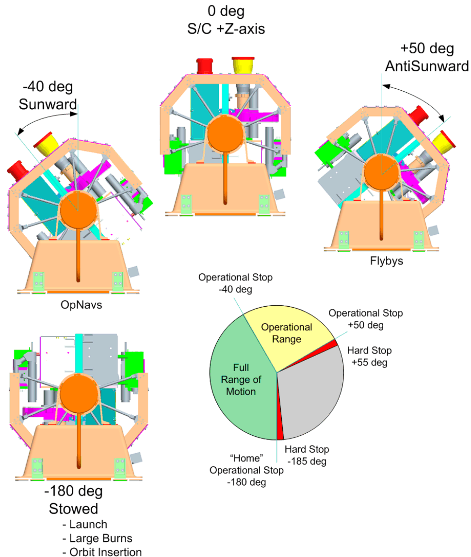
Figure 6: Range of motion of the MDIS pivot platform. Operational range is -40^\circ sunward to +50^\circ antisunward (planetward). When stowed, the sensitive first optic of each telescope is protected.
