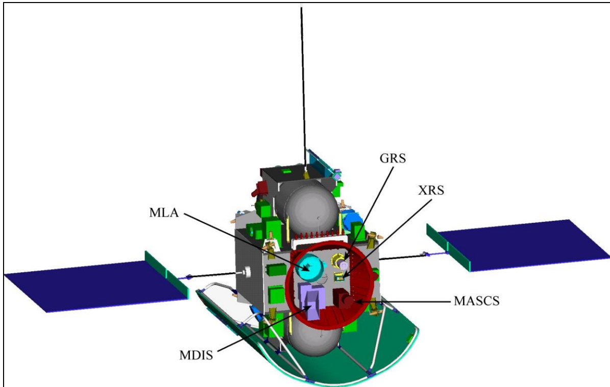
Figure 4: MESSENGER instrument deck showing instrument accommodation.
