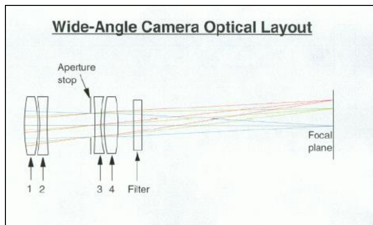
Figure 11. WAC optical layout.
