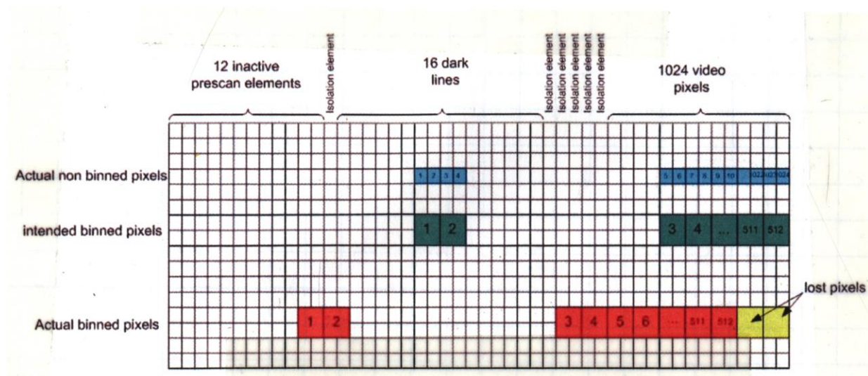
Figure 13. Pixels intended for dark columns, and actual pixels used in binned images for WAC and NAC.
