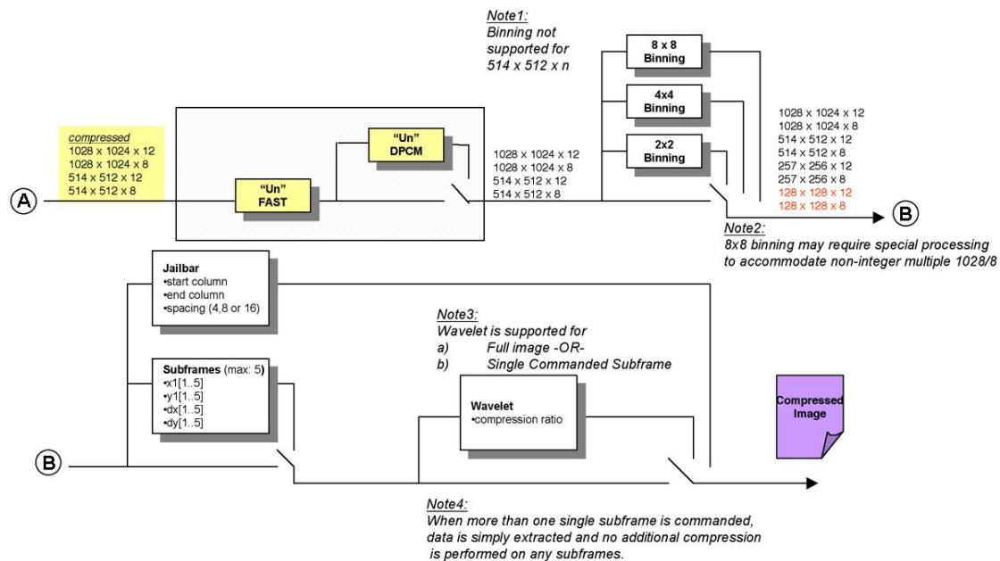
Figure 7b MESSENGER Main Processor (MP) image post-processing compression flowchart.
