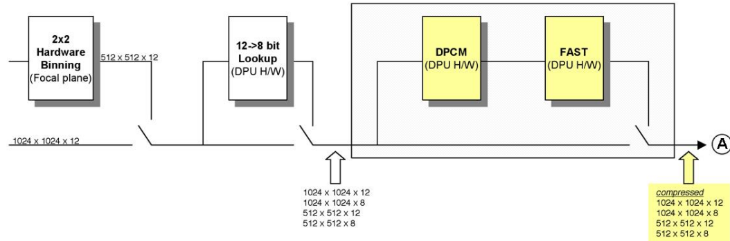
Figure 7a MDIS/DPU real-time compression flowchart
